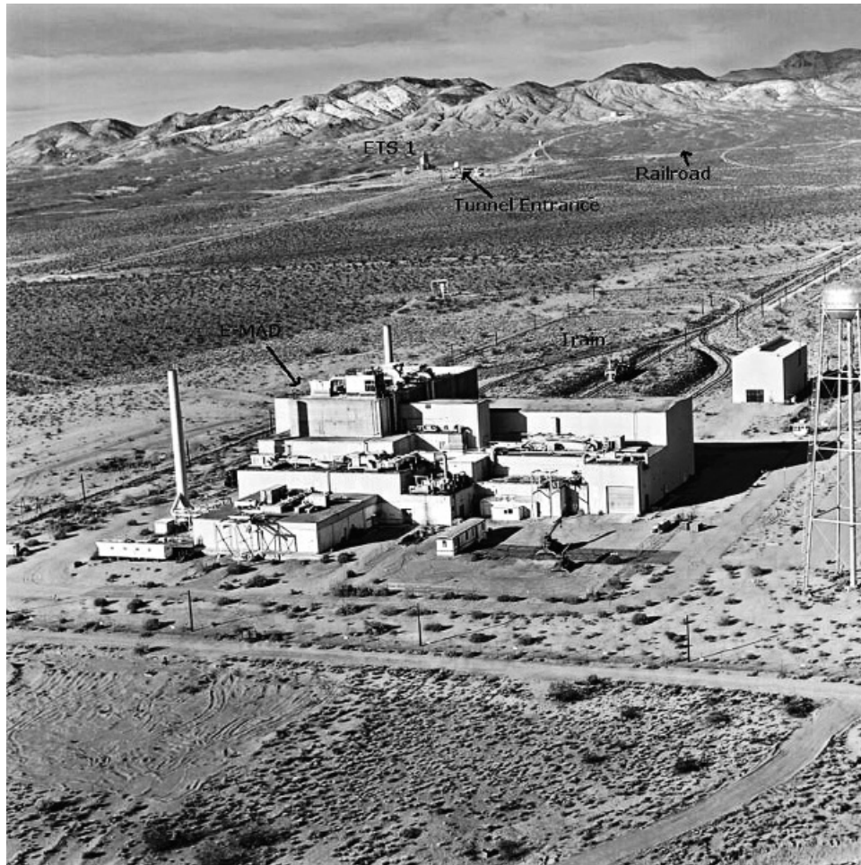
The Nuclear Rocket Test Facility at Jackass Flats, located in Area 25, seen here from above sometime in the 1960s. Three test cells (ETS-1, E-MAD, and R-MAD) were connected by a remote-controlled railroad that transported the highly radioactive reactor between them. ( Department of Energy )
