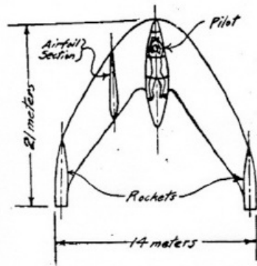
Plan View of HORTEN Airplane
